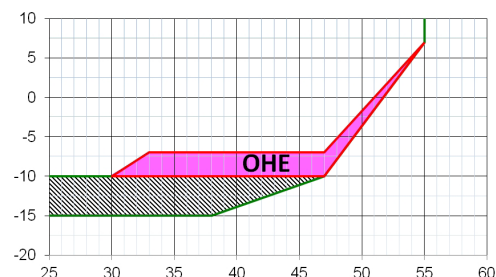
4-pipe configuration - Extended operating range with OHE kit
