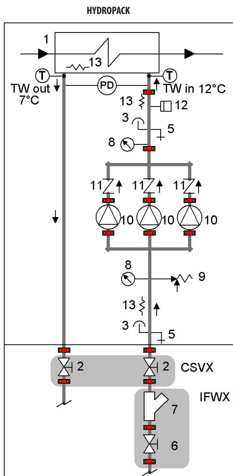
Illustrative diagram referred to unit size 240.4 with HydroPack with no. 3 of pumps
