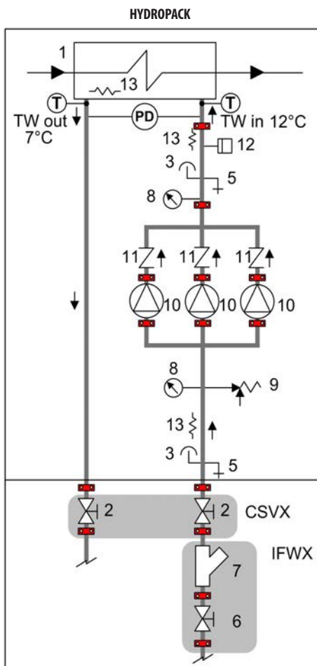
Illustrative diagram referred to unit size 240.4 with Hydronic with no. 3 of pumps
